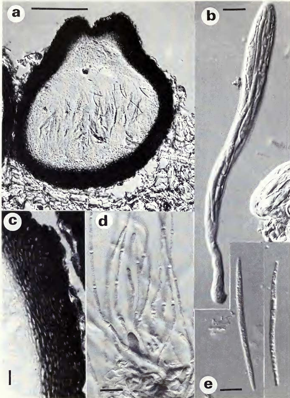
Fig. 44 Cresporhaphis macrospora (Eitner) Aguirre (W 19701–lectotype) (a) Vertical section of ascoma; scale = 100 \mu\text{m} ; (b) Ascus and ascospores biserially arranged; (c) Detail of exciple: textura angularis to prismatica; (d) Paraphyses; (e) Ascospores; scale = 10 \mu\text{m} .
